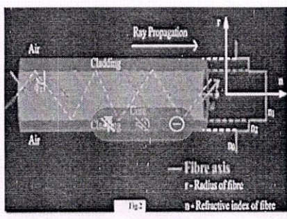
Fig: 2) Multimode step index optical fiber
